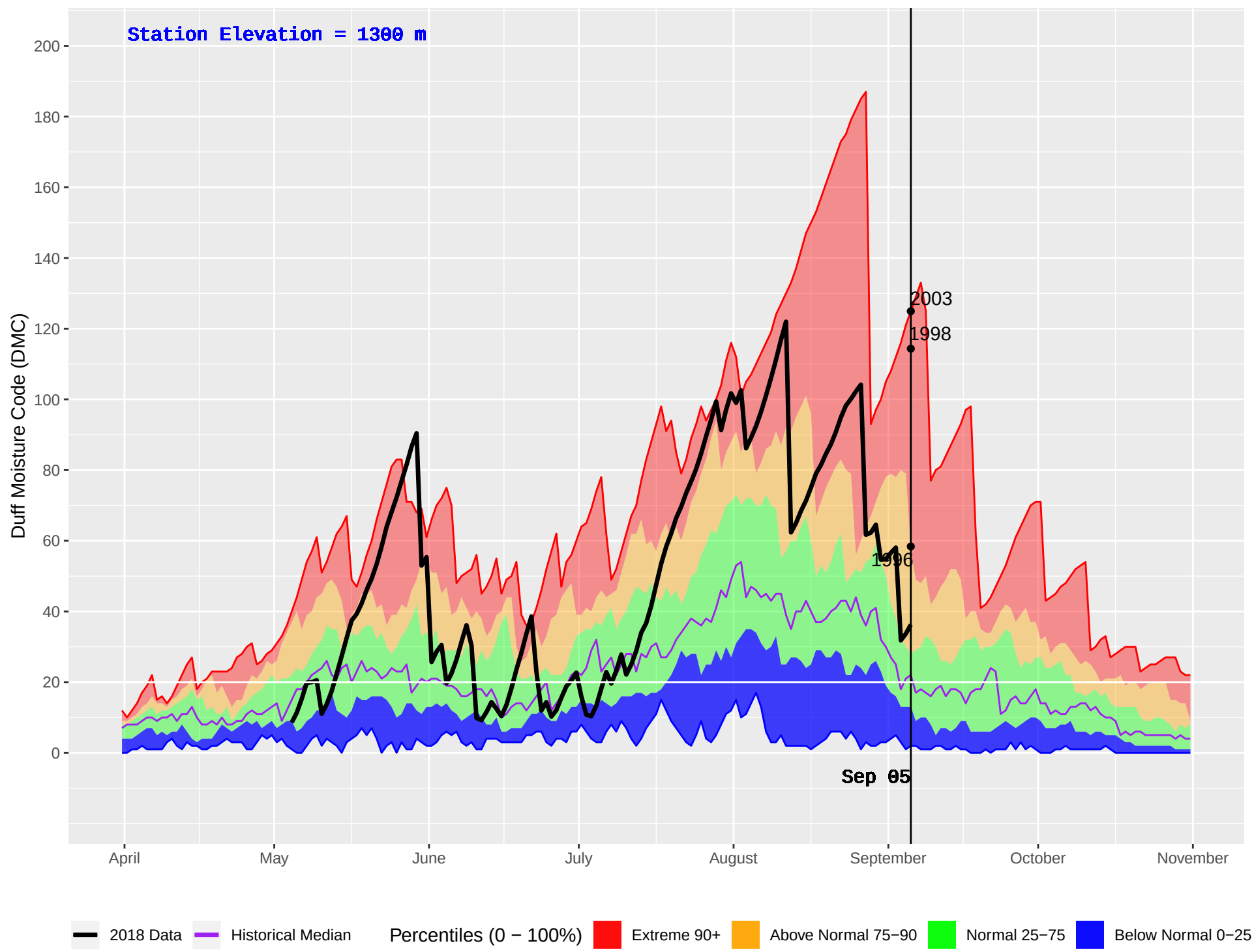
MARION (367) : Historical (1994–2016) and Current (2018) Daily Duff Moisture Code (DMC)
